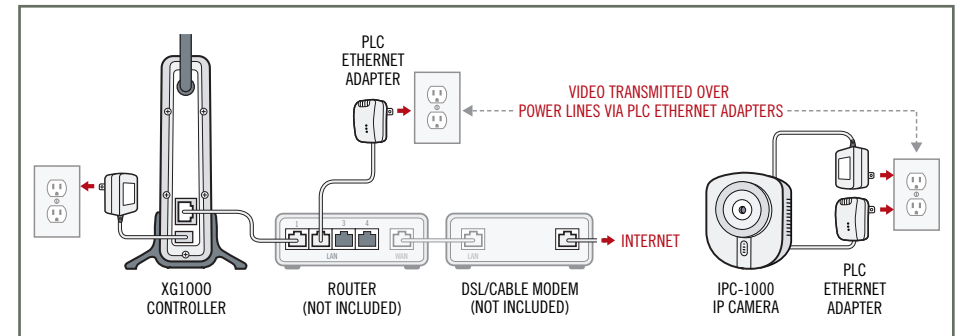
COMPLETED CONFIGURATION USING OPTIONAL PLC ETHERNET ADAPTERS (SOLD SEPARATELY)
